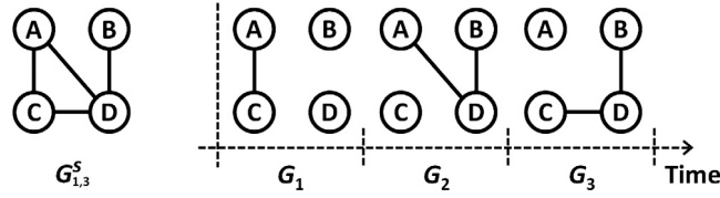
Fig. 3. An example of the dynamic network. (Left) aggregated static network. (Right) time-varying dynamic network. After [69].
