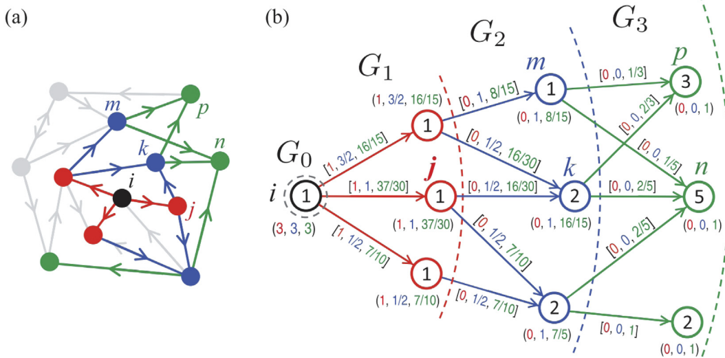
Fig. 4. The calculation of the range-limited betweenness centrality. (a) An example of toy network. The three successive shells of C_3 subnetwork of node i are colored red, blue, green. Gray elements are not part of subnetwork. (b) The b_l^r(i|j) values are corresponding for shells l = 1, l = 2 , and l = 3 . After [71].
